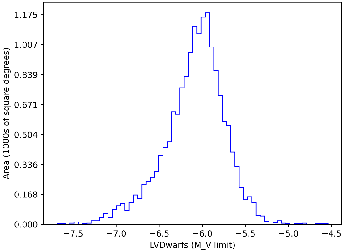
baseline_v4.0_10yrs gi: LVDwarfs
