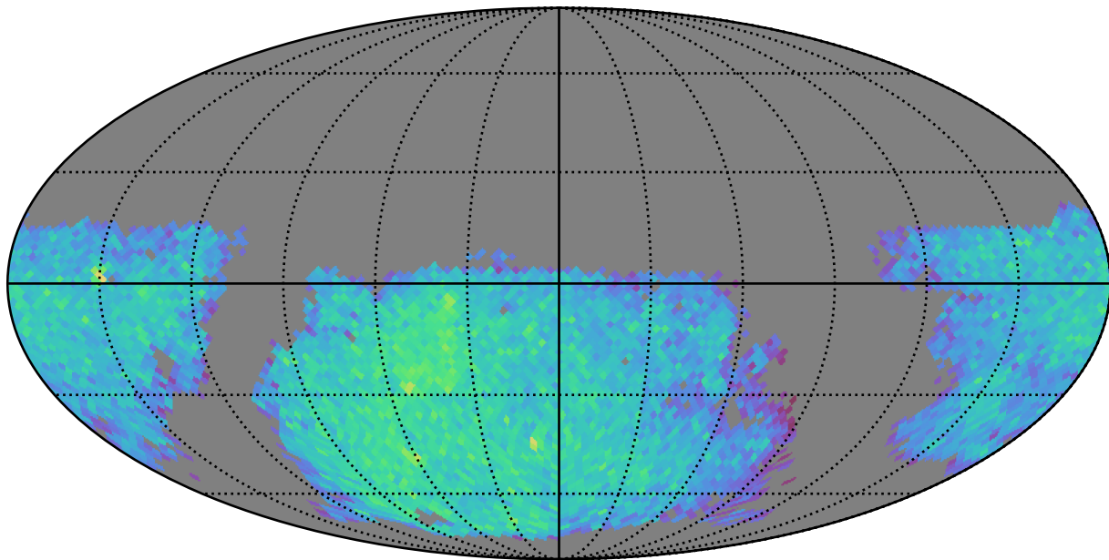
baseline_v4.0_10yrs gi: LVDwarfs
