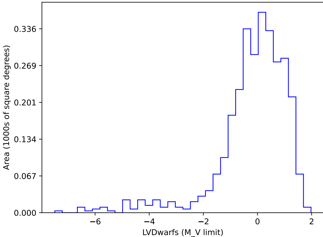
baseline_v4.0_10yrs gi SCP: LVDwarfs
