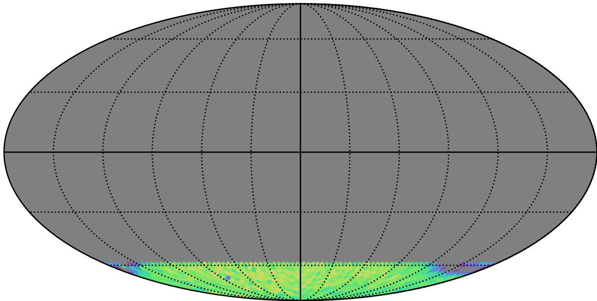
baseline_v4.0_10yrs gi SCP: LVDwarfs
