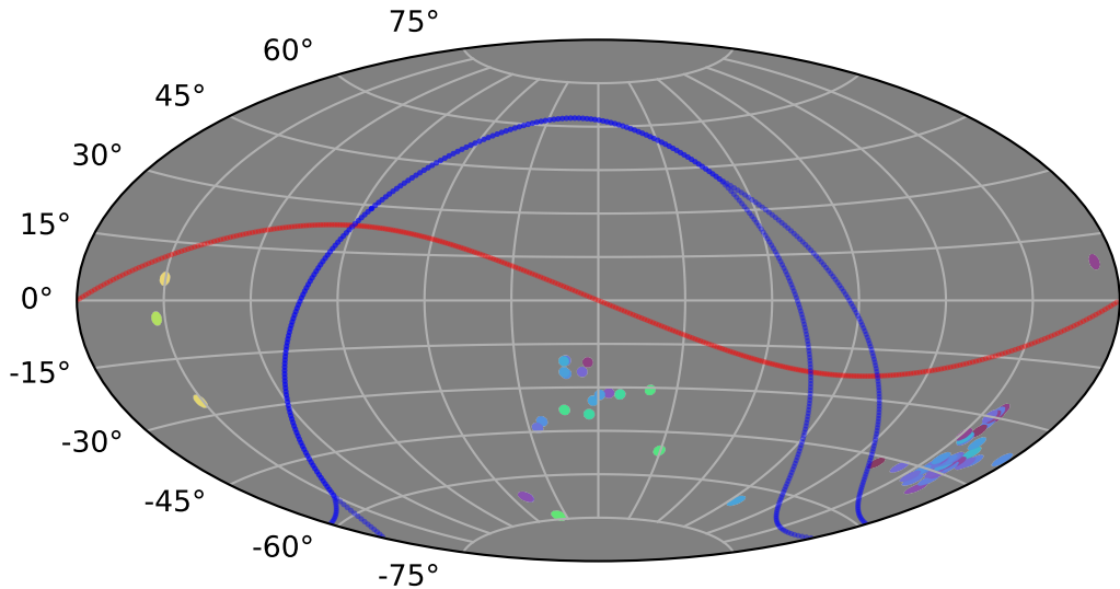
baseline_v4.0_10yrs gi: LVDwarfs
