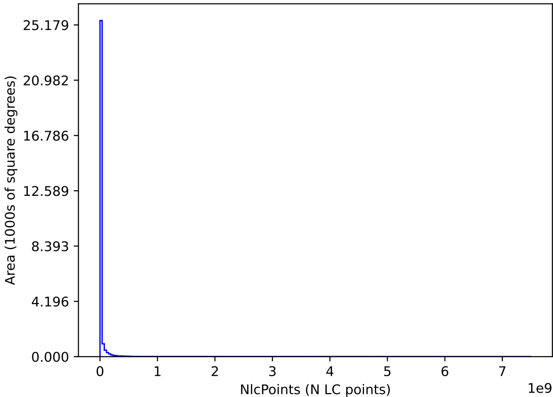
baseline_v4.0_10yrs : NlcPoints
