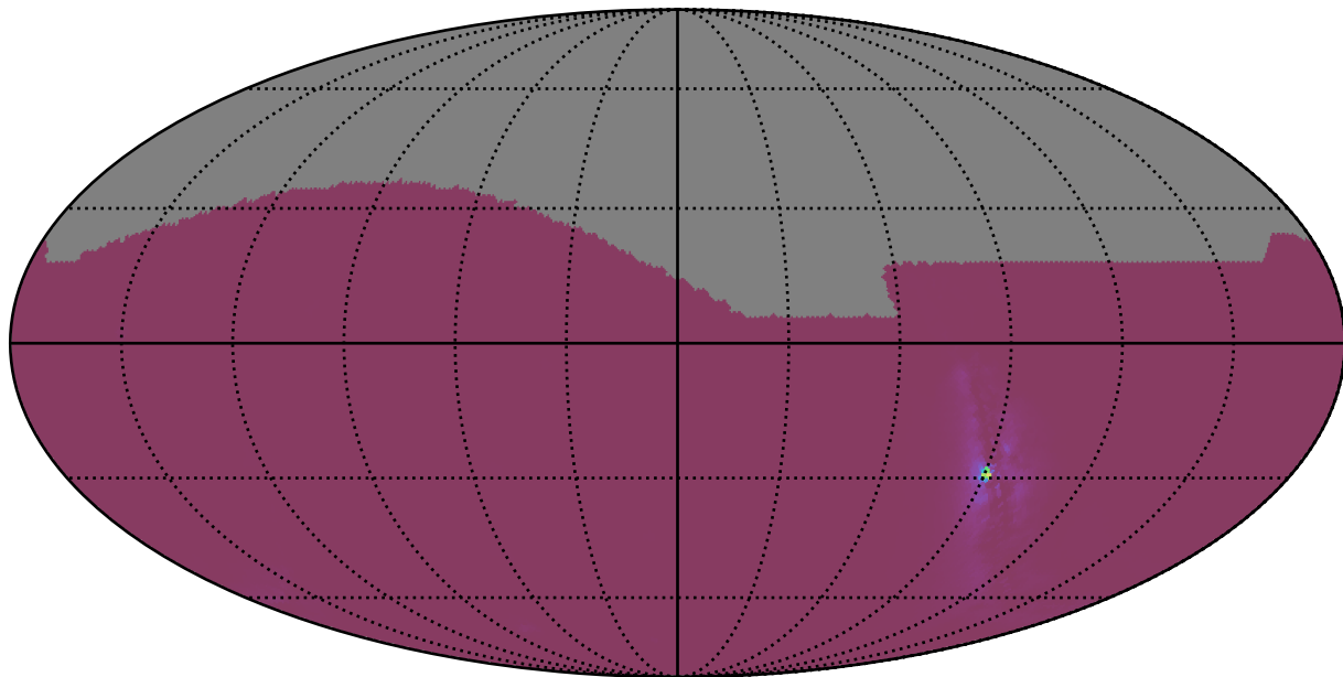
baseline_v4.0_10yrs : NlcPoints
