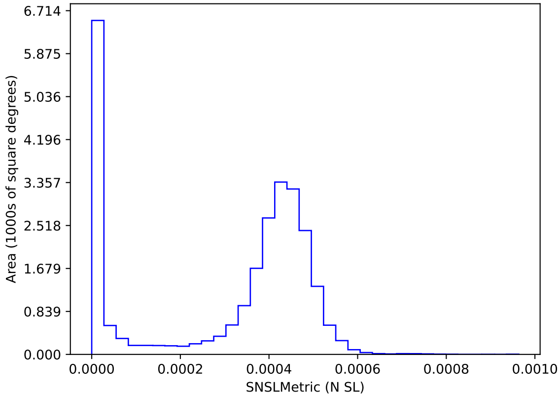
baseline_v4.0_10yrs : SNSLMetric
