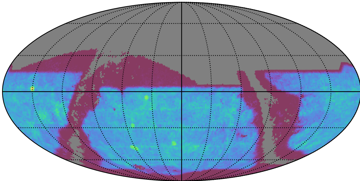
baseline_v4.0_10yrs : SNSLMetric
