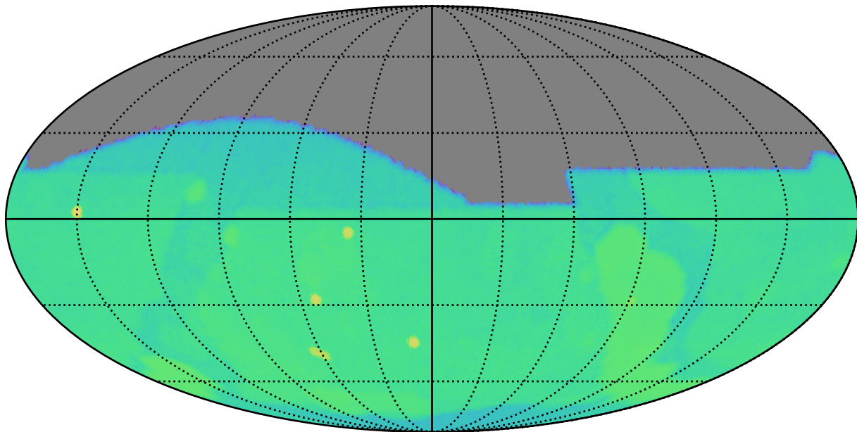
baseline_v4.0_10yrs g: SurfaceBrightLimit
