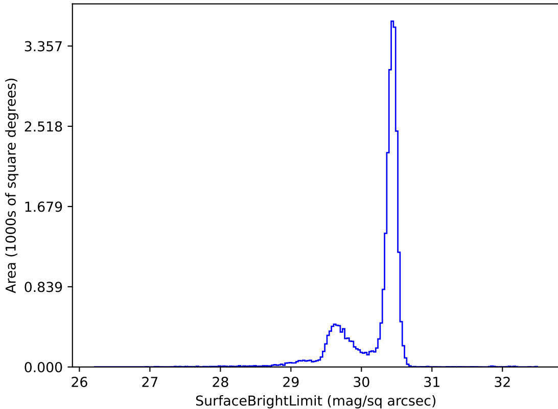
baseline_v4.0_10yrs r: SurfaceBrightLimit
