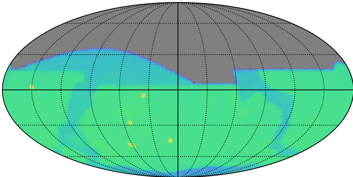
baseline_v4.0_10yrs r: SurfaceBrightLimit
