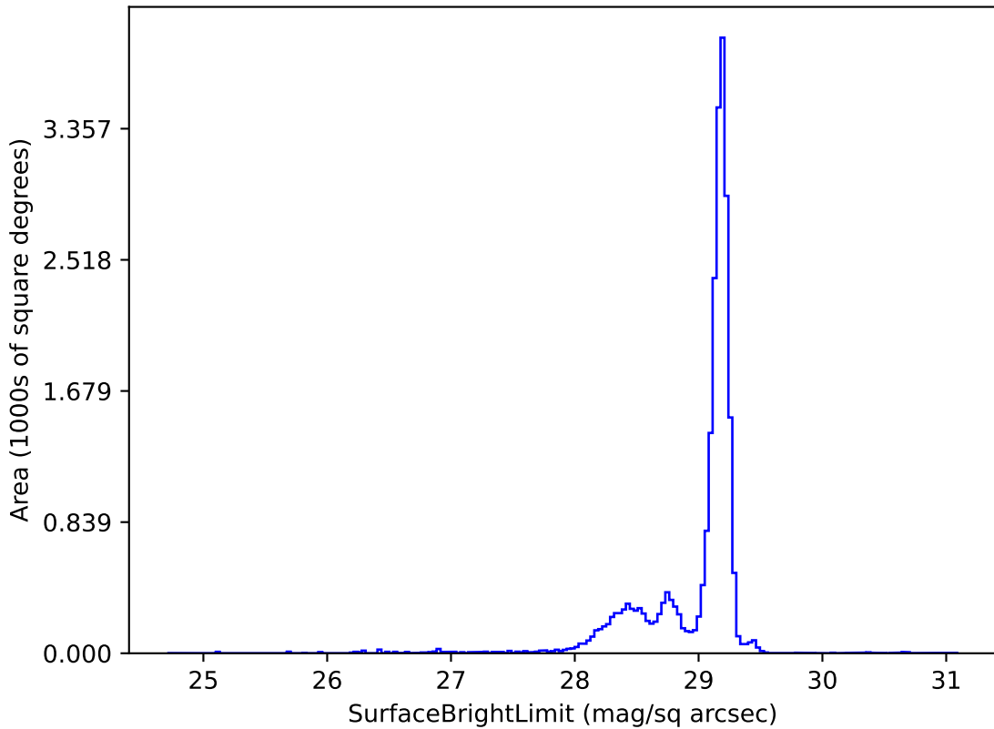
baseline_v4.0_10yrs u: SurfaceBrightLimit
