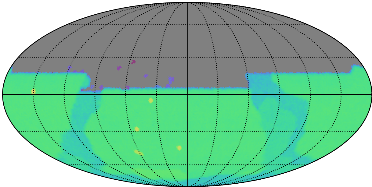
baseline_v4.0_10yrs u: SurfaceBrightLimit
