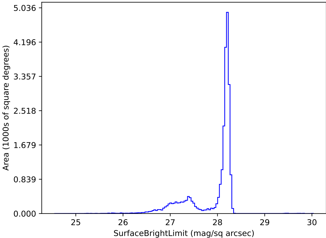
baseline_v4.0_10yrs y: SurfaceBrightLimit
