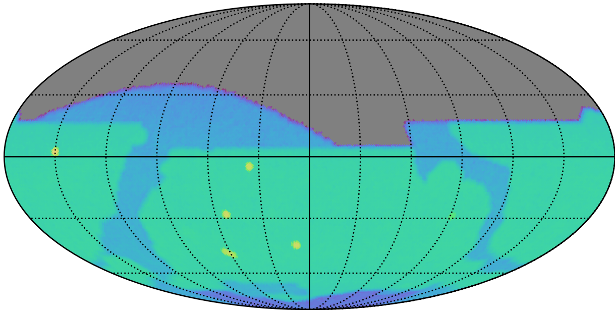
baseline_v4.0_10yrs z: SurfaceBrightLimit
