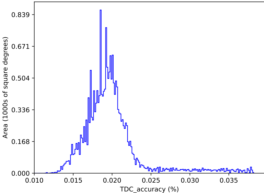
baseline_v4.0_10yrs : TDC_accuracy
