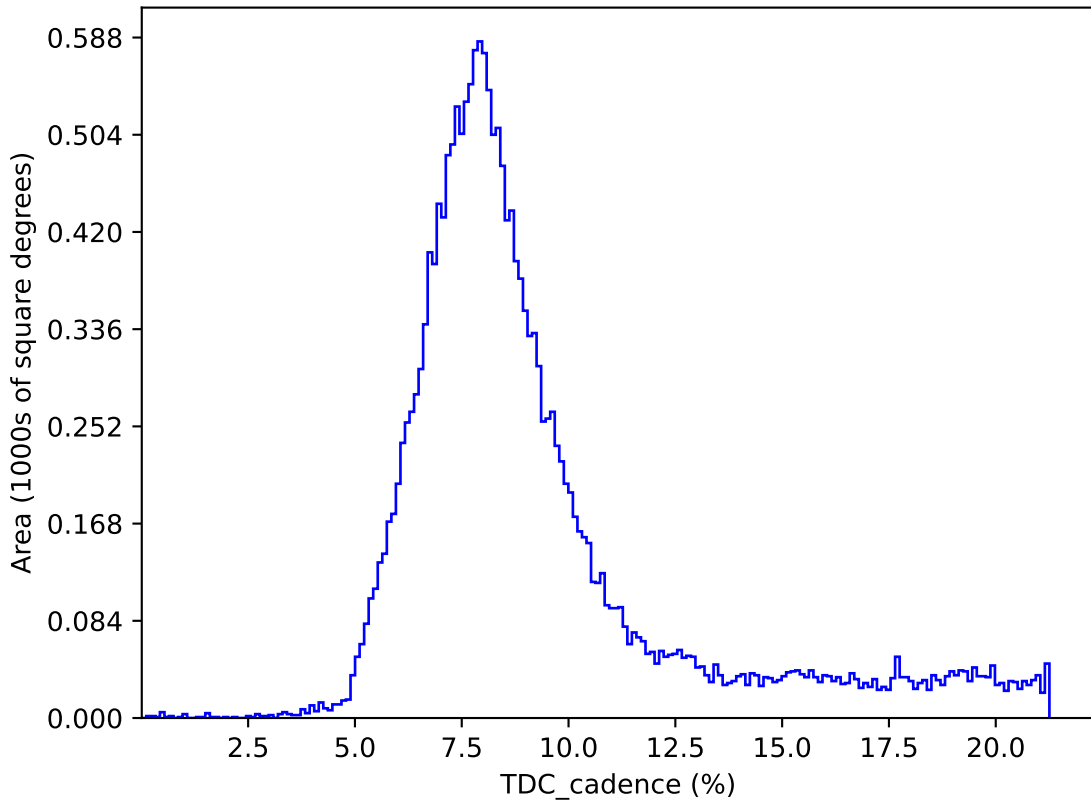
baseline_v4.0_10yrs : TDC_cadence
