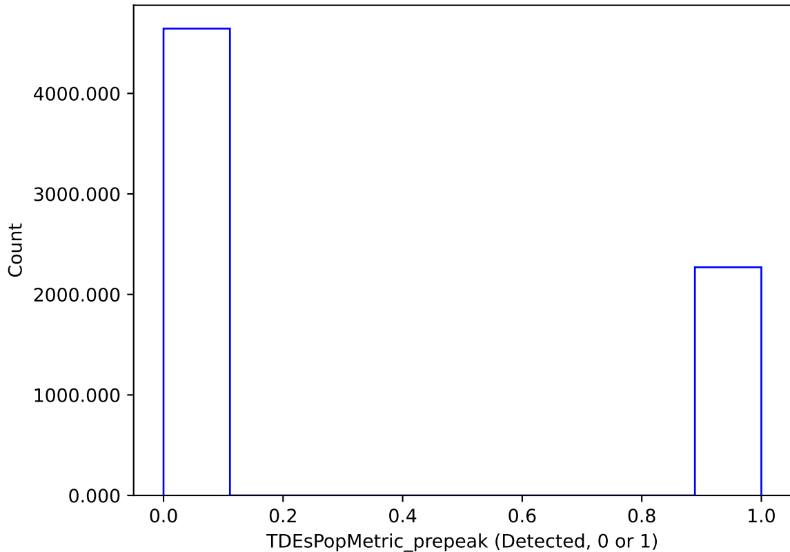
baseline_v4.0_10yrs : TDEsPopMetric_prepeak
