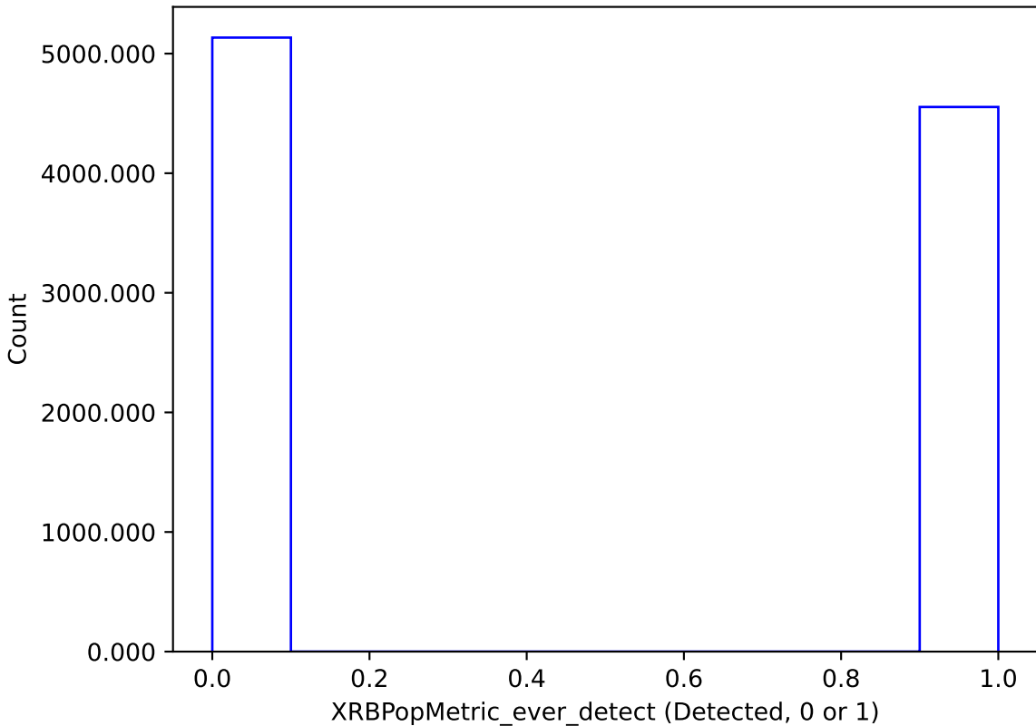
baseline_v4.0_10yrs : XRBPoMetric_ever_detect
