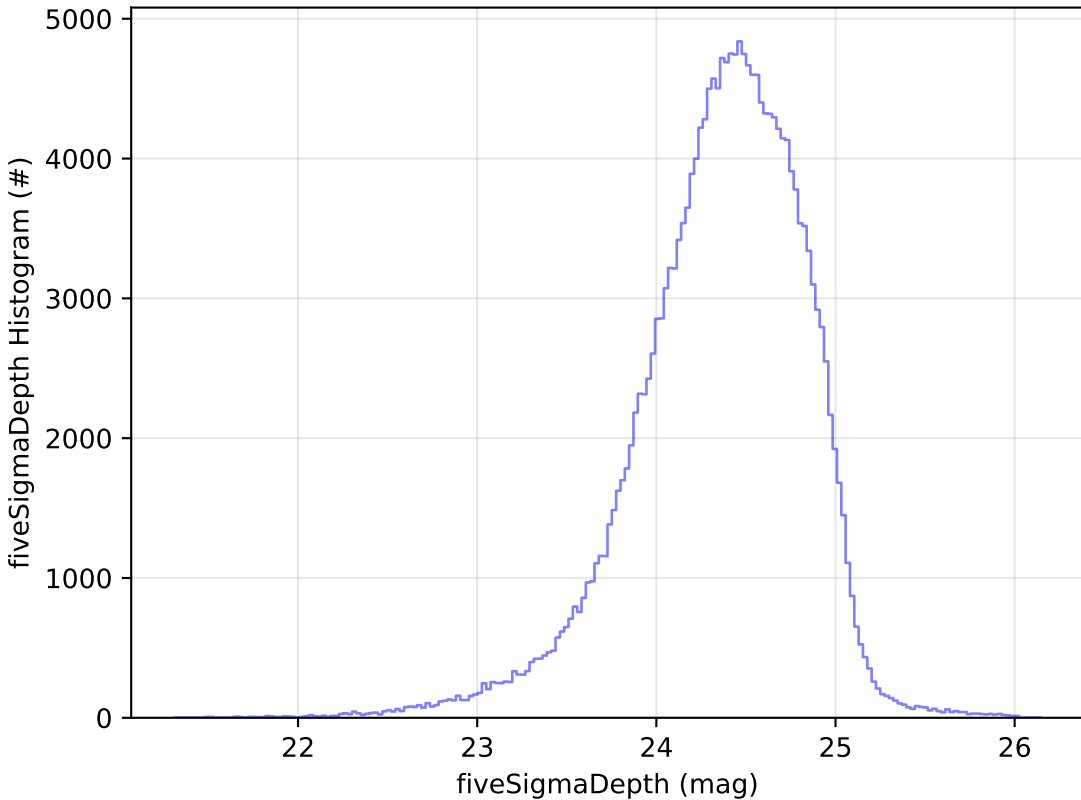
baseline_v4.0_10yrs g: fiveSigmaDepth Histogram
