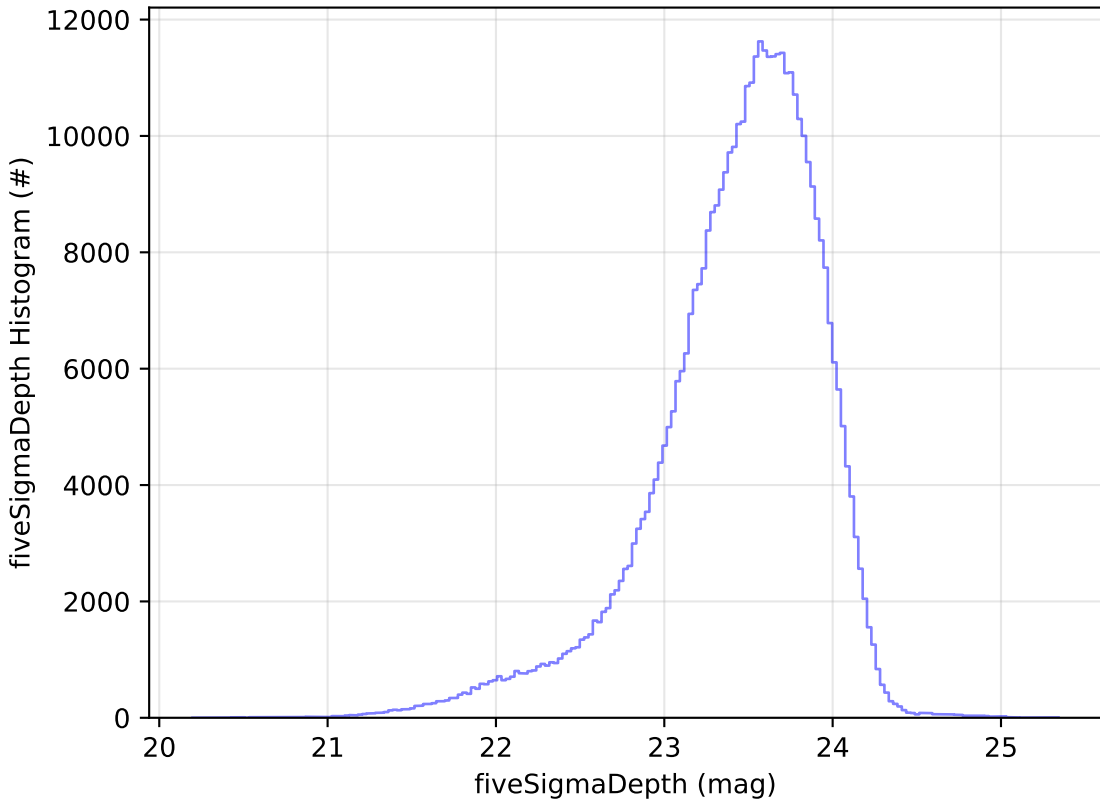
baseline_v4.0_10yrs i: fiveSigmaDepth Histogram
