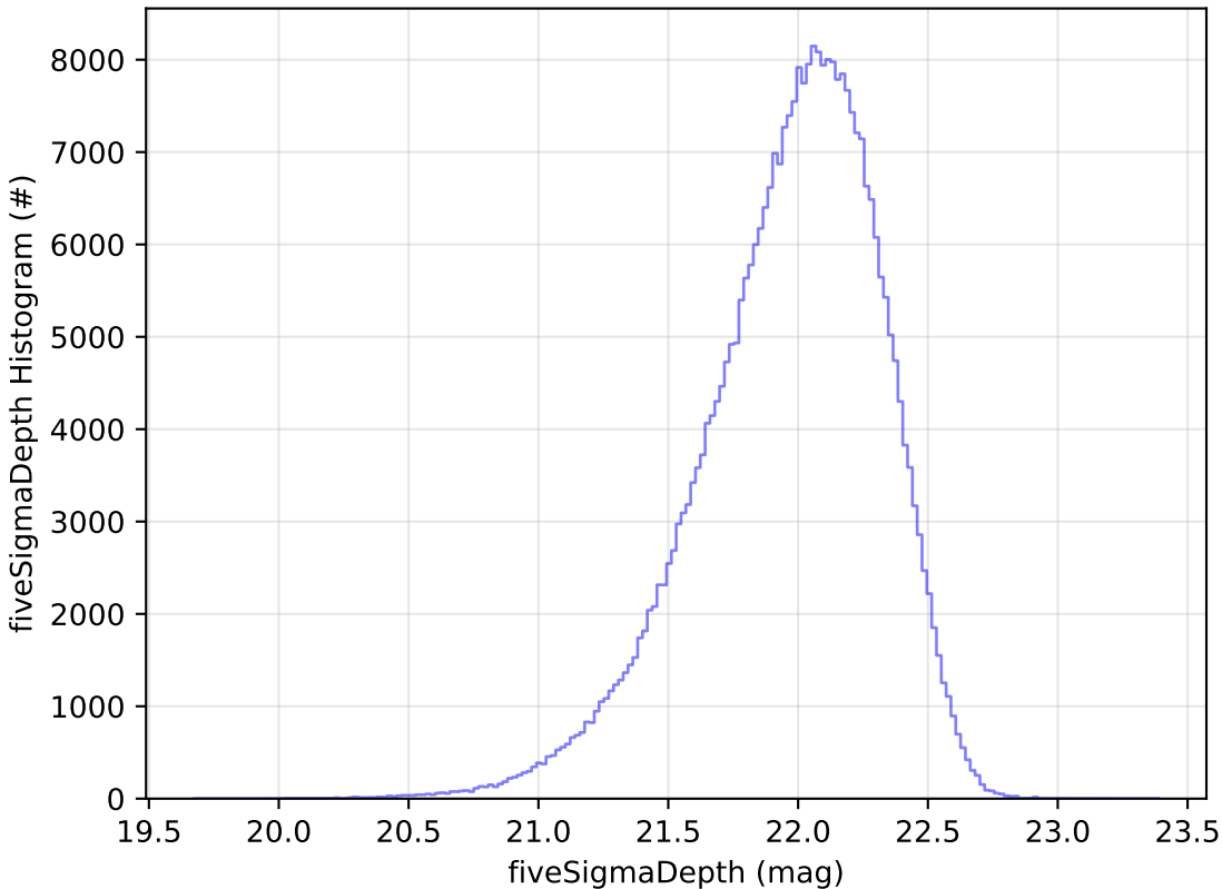
baseline_v4.0_10yrs y: fiveSigmaDepth Histogram
