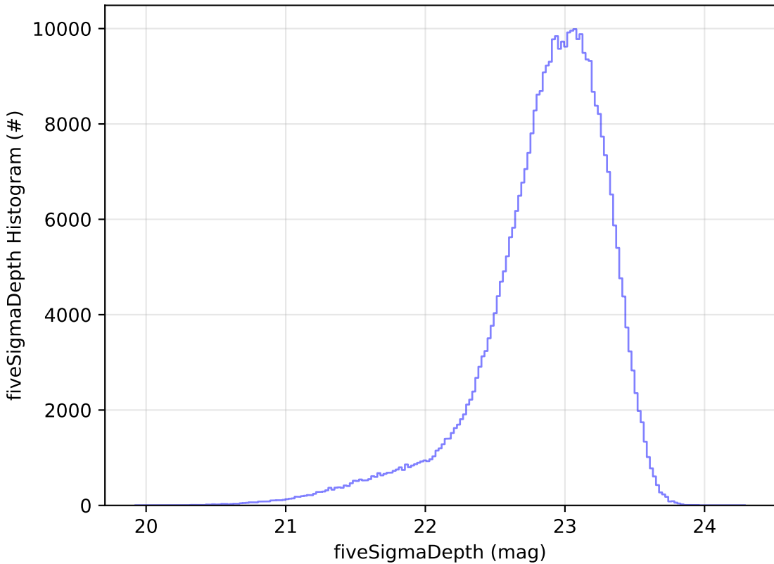
baseline_v4.0_10yrs z: fiveSigmaDepth Histogram
