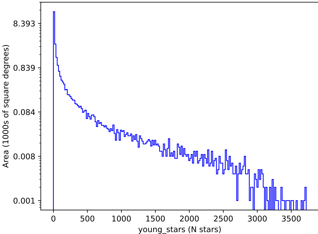
baseline_v4.0_10yrs : young_stars
