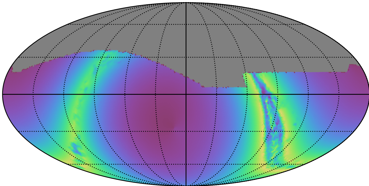
baseline_v4.0_10yrs : young_stars
