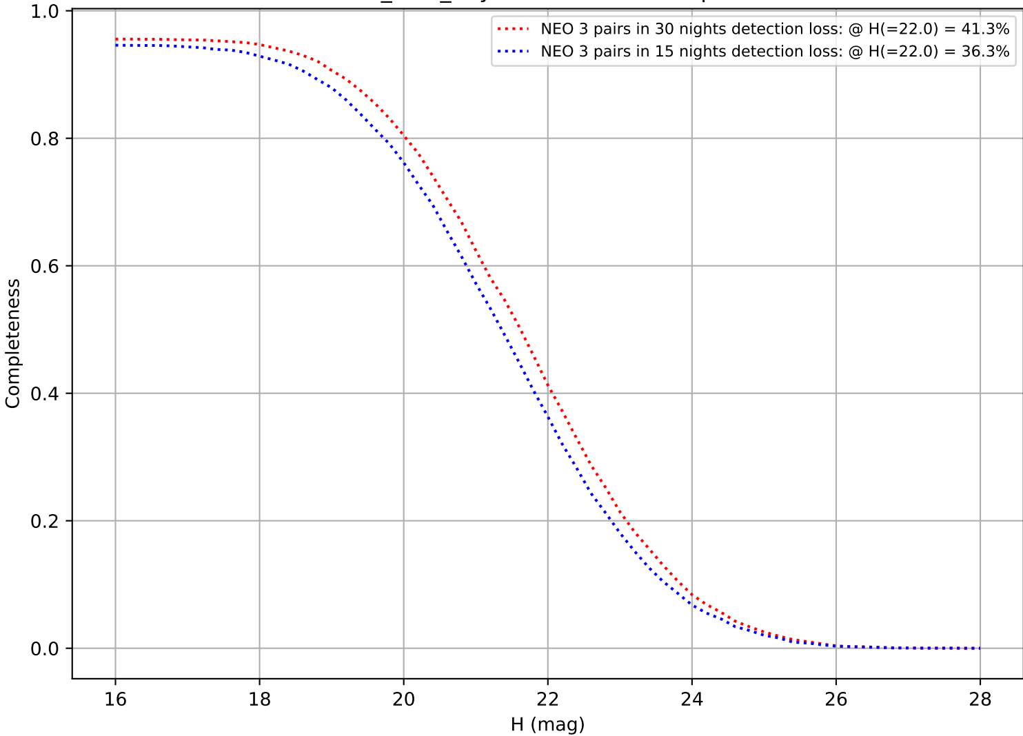
baseline_v4.0_10yrs: DifferentialCompleteness
