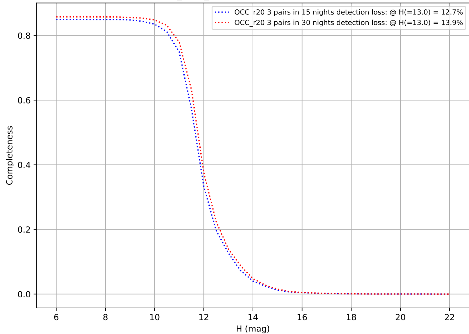
baseline_v4.0_10yrs: DifferentialCompleteness
