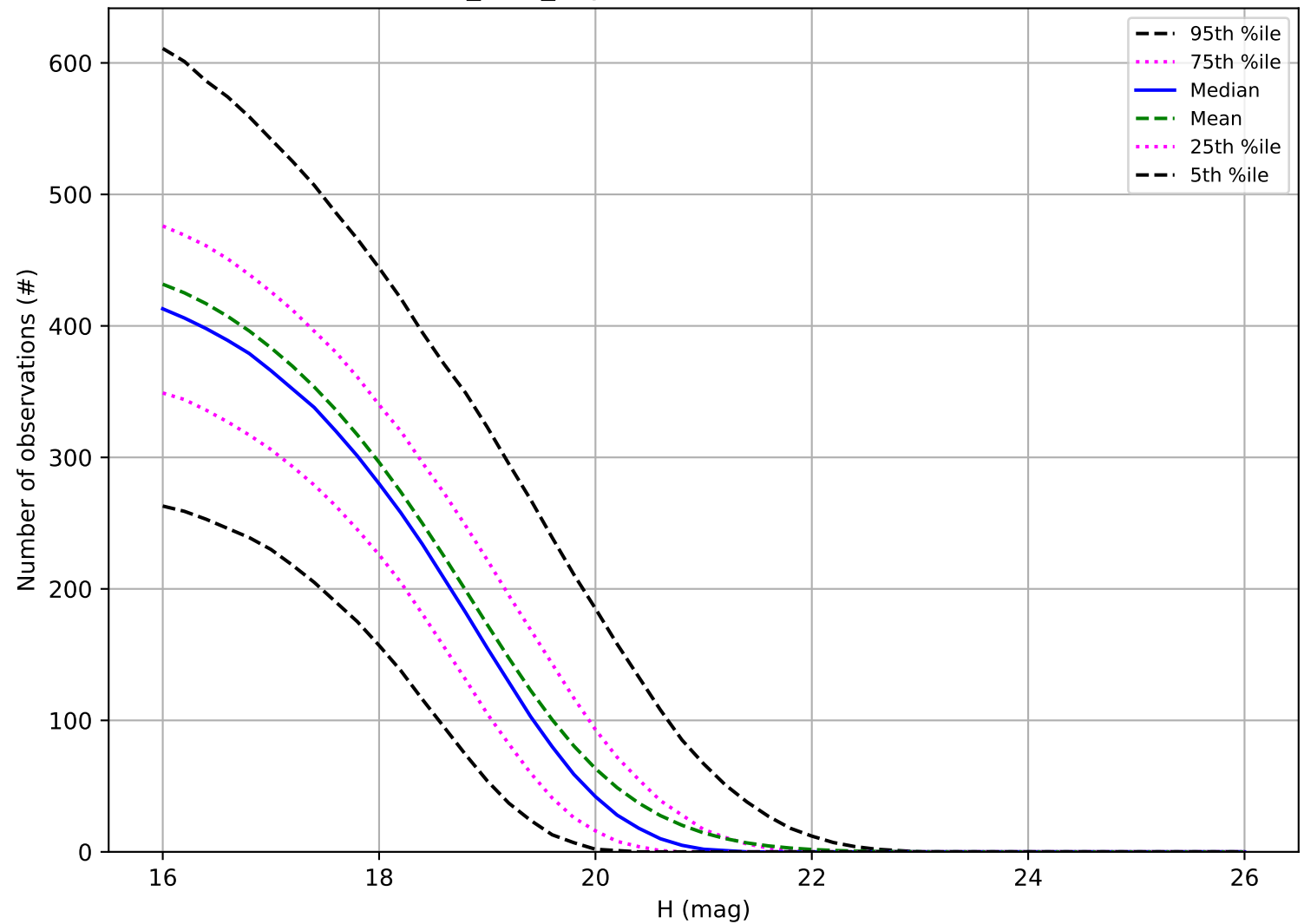
baseline_v4.0_10yrs: Number of observations MBA
