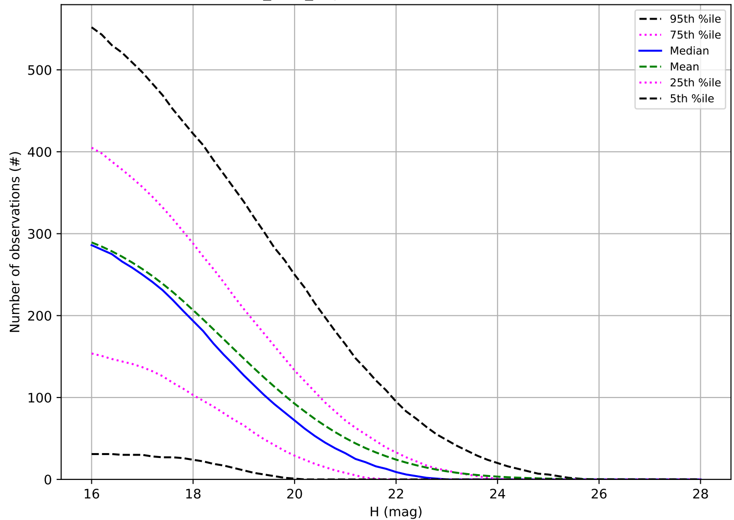
baseline_v4.0_10yrs: Number of observations NEO
