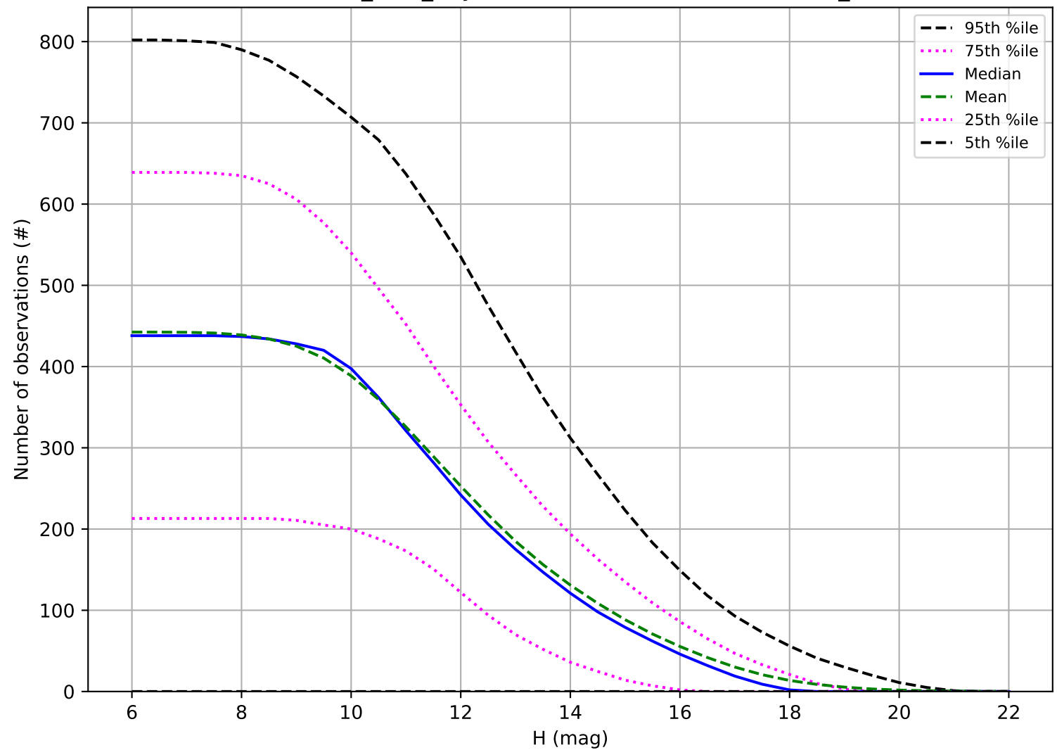
baseline_v4.0_10yrs: Number of observations OCC_r5
