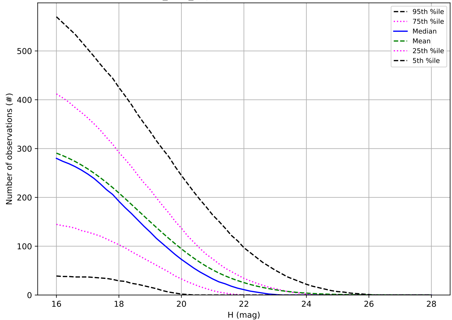
baseline_v4.0_10yrs: Number of observations PHA
