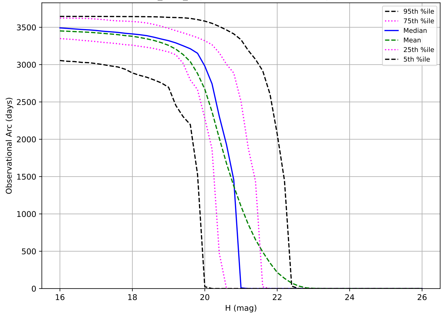
baseline_v4.0_10yrs: Observational Arc Length MBA
