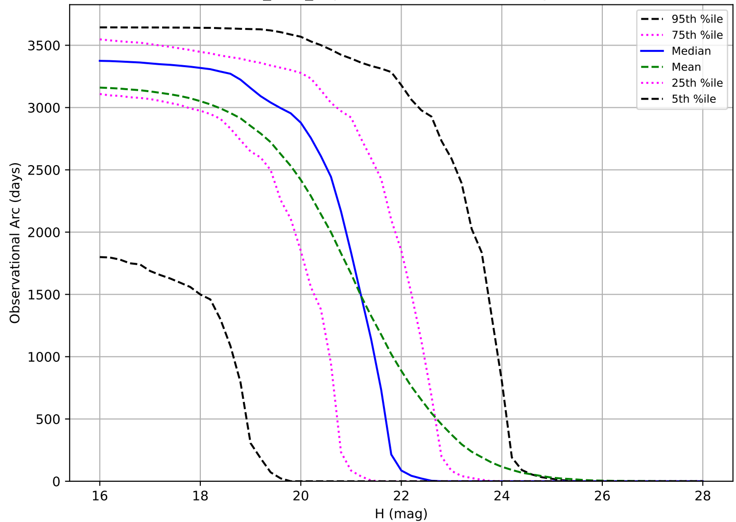
baseline_v4.0_10yrs: Observational Arc Length NEO
