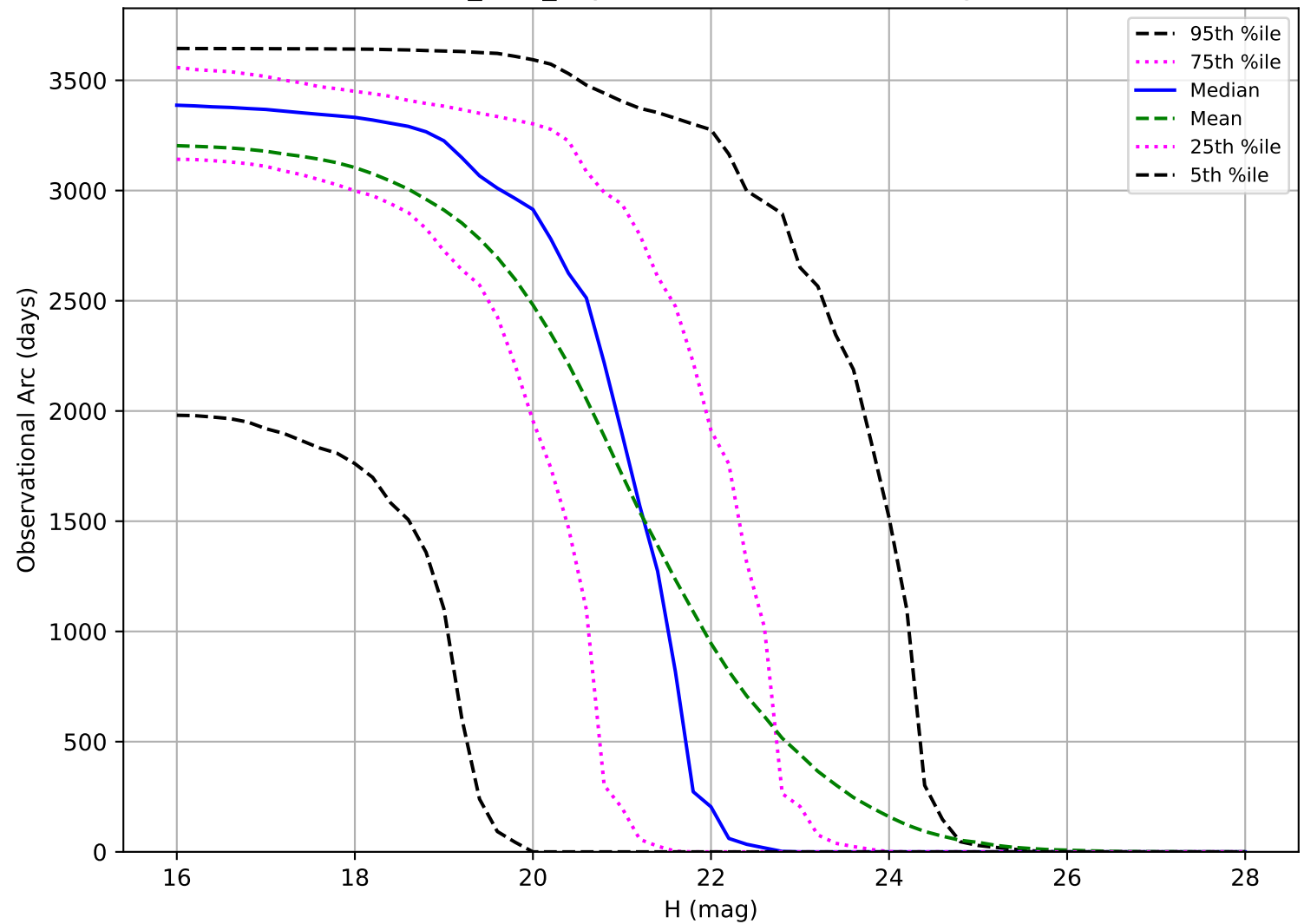
baseline_v4.0_10yrs: Observational Arc Length PHA
