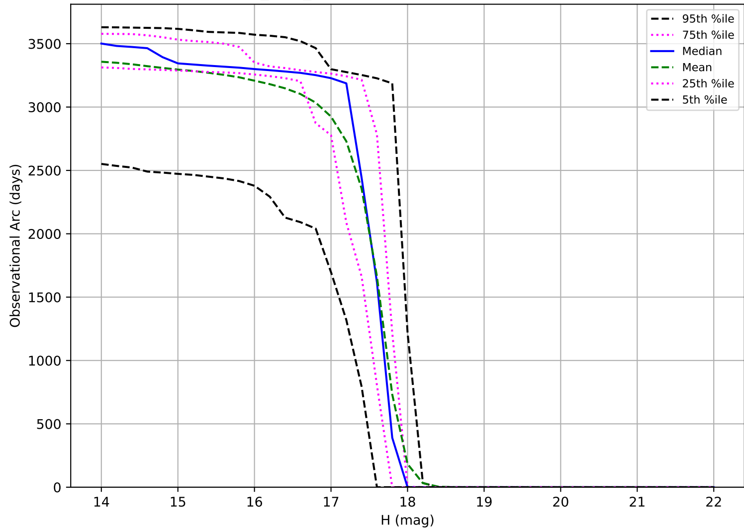
baseline_v4.0_10yrs: Observational Arc Length Trojan
