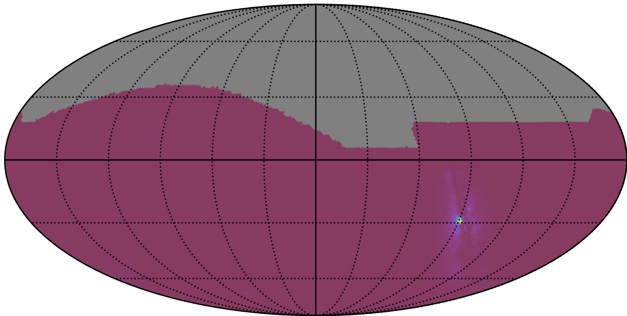
ddf_agn_v3.5_10yrs : NlcPoints
