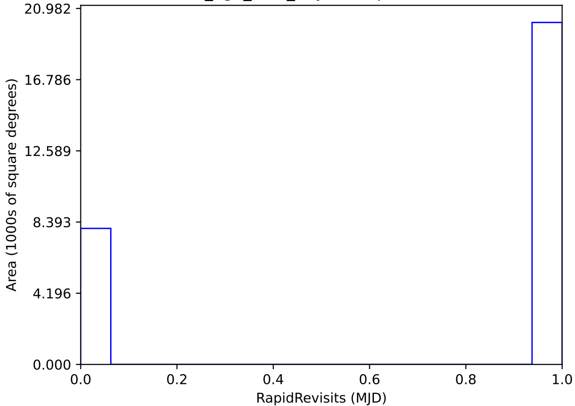
ddf_agn_v3.5_10yrs : RapidRevisits
