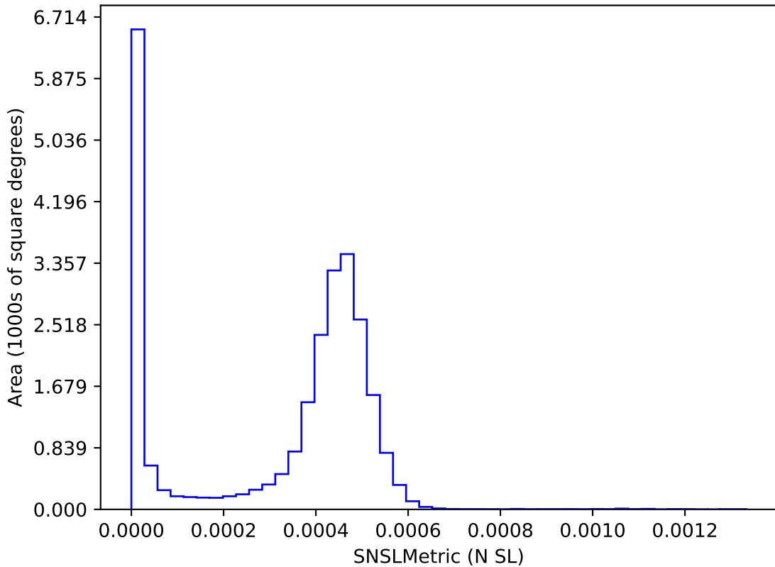
ddf_agn_v3.5_10yrs : SNSLMetric
