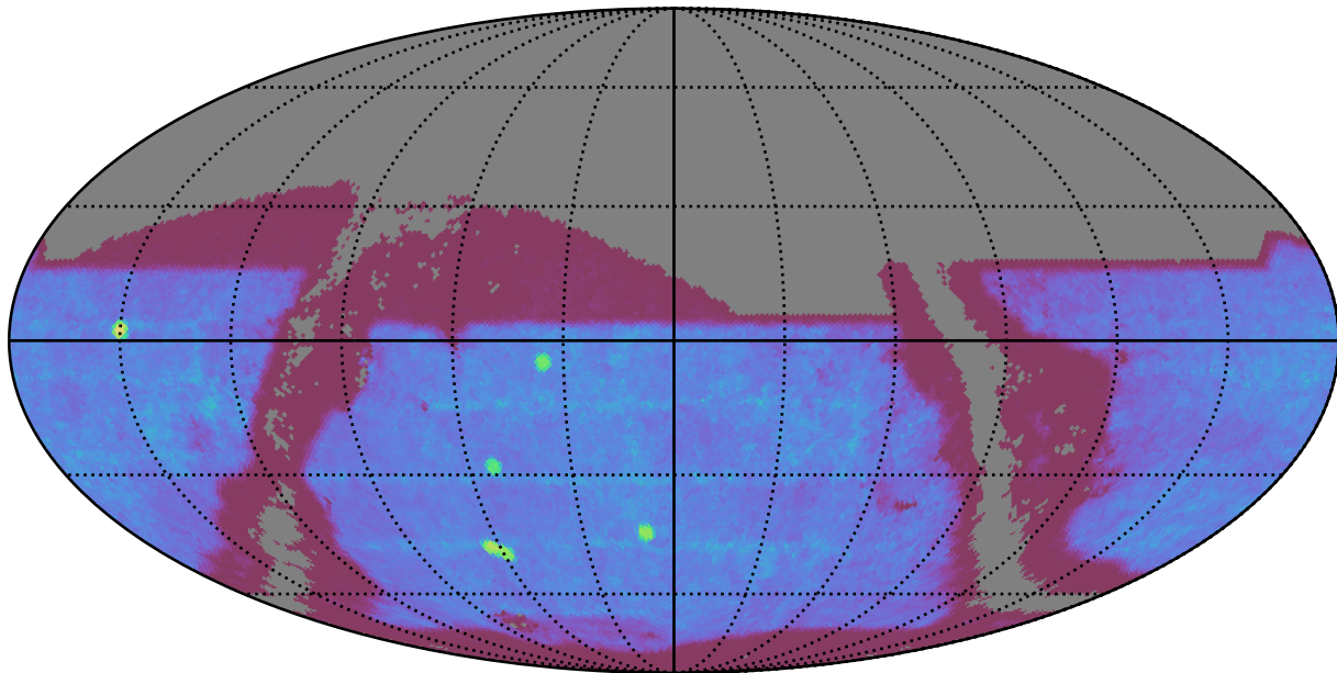
ddf_agn_v3.5_10yrs : SNSLMetric
