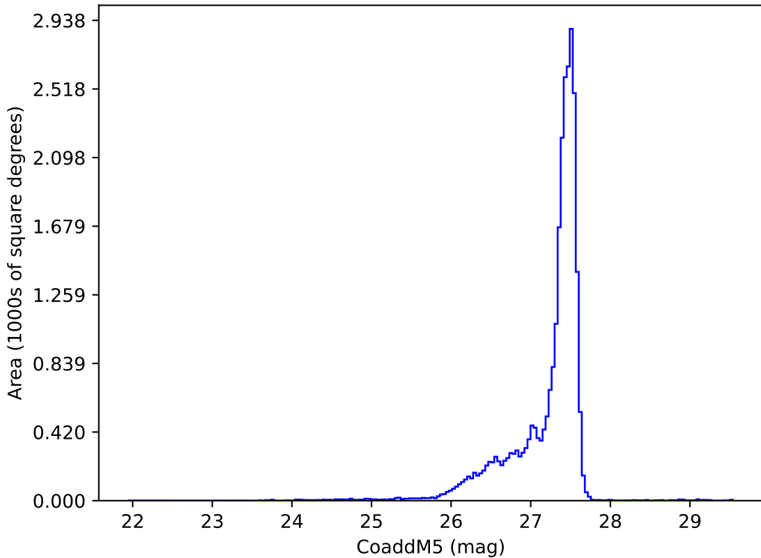
ddf_roll_v3.5_10yrs : CoaddM5
