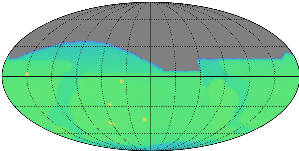
ddf_roll_v3.5_10yrs : CoaddM5
