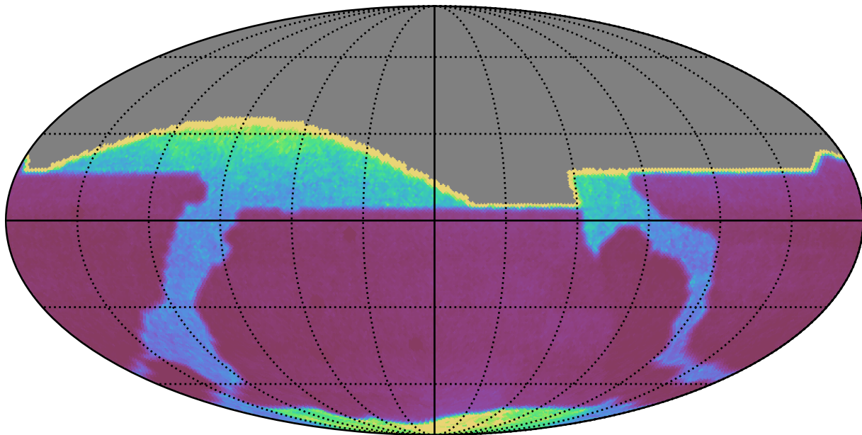
ddf_roll_v3.5_10yrs : properMotion
