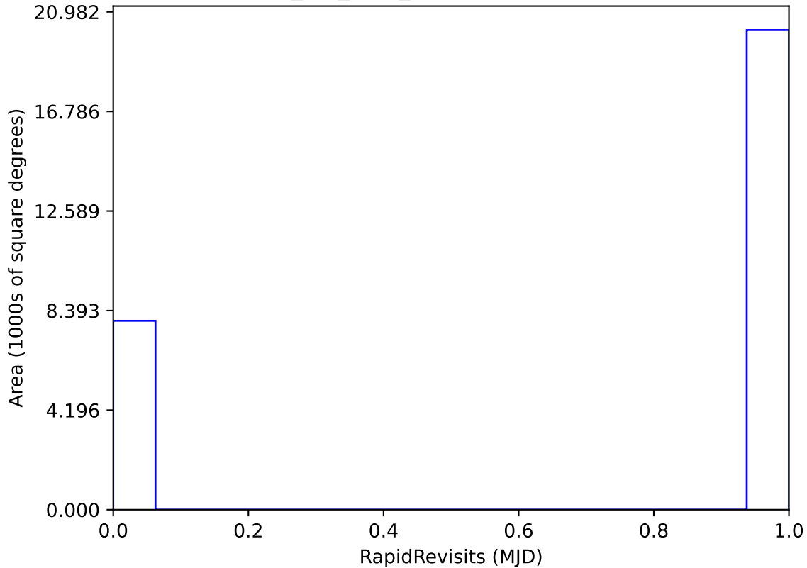
ddf_roll_v3.5_10yrs : RapidRevisits
