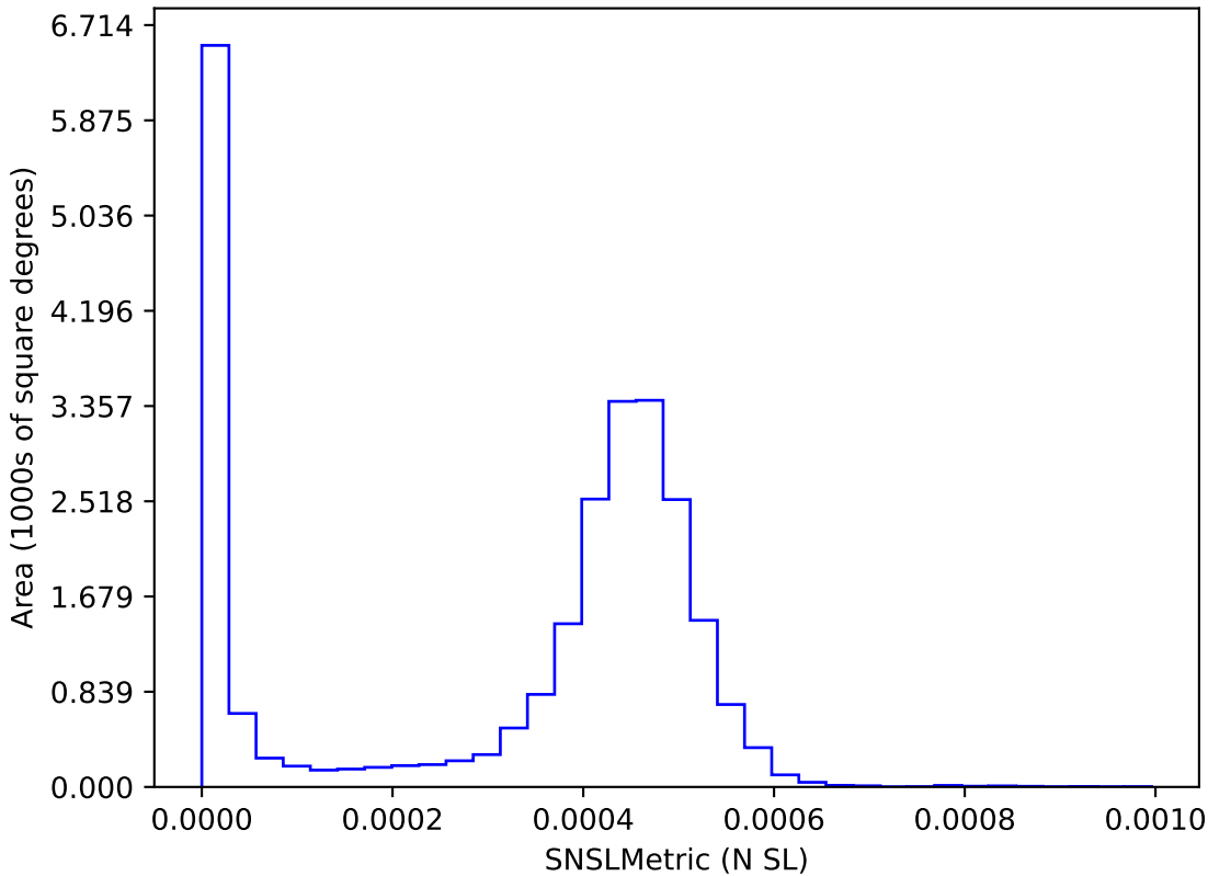
ddf_roll_v3.5_10yrs : SNSLMetric
