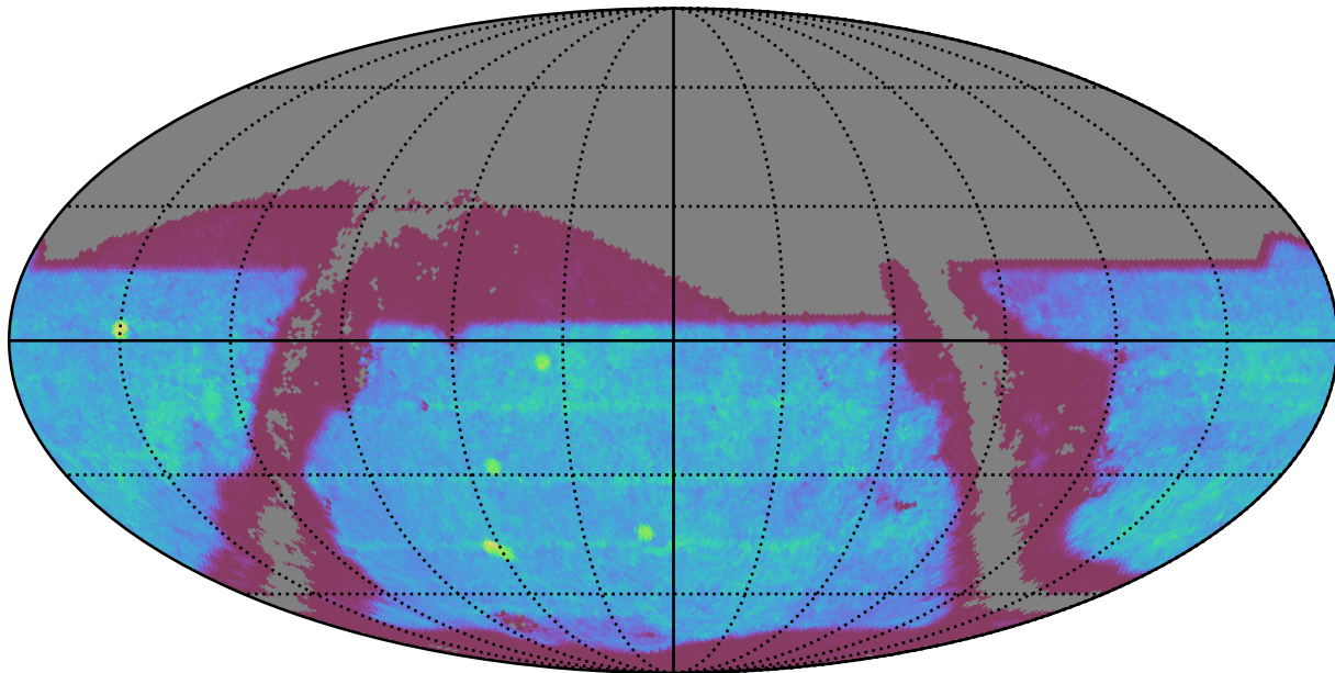
ddf_roll_v3.5_10yrs : SNSLMetric
