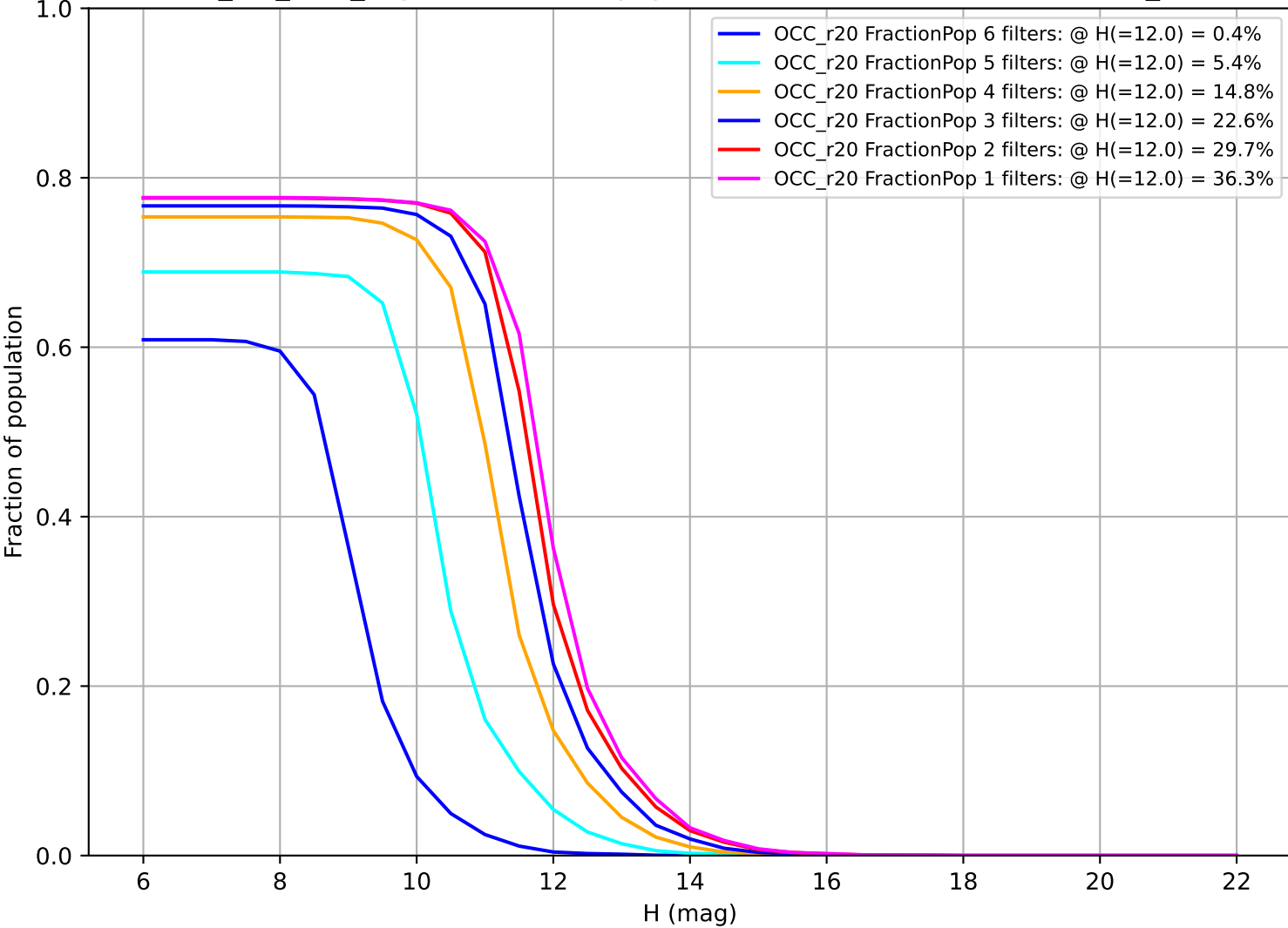
ddf_roll_v3.5_10yrs: Fraction of population with colors in X filters OCC_r20
