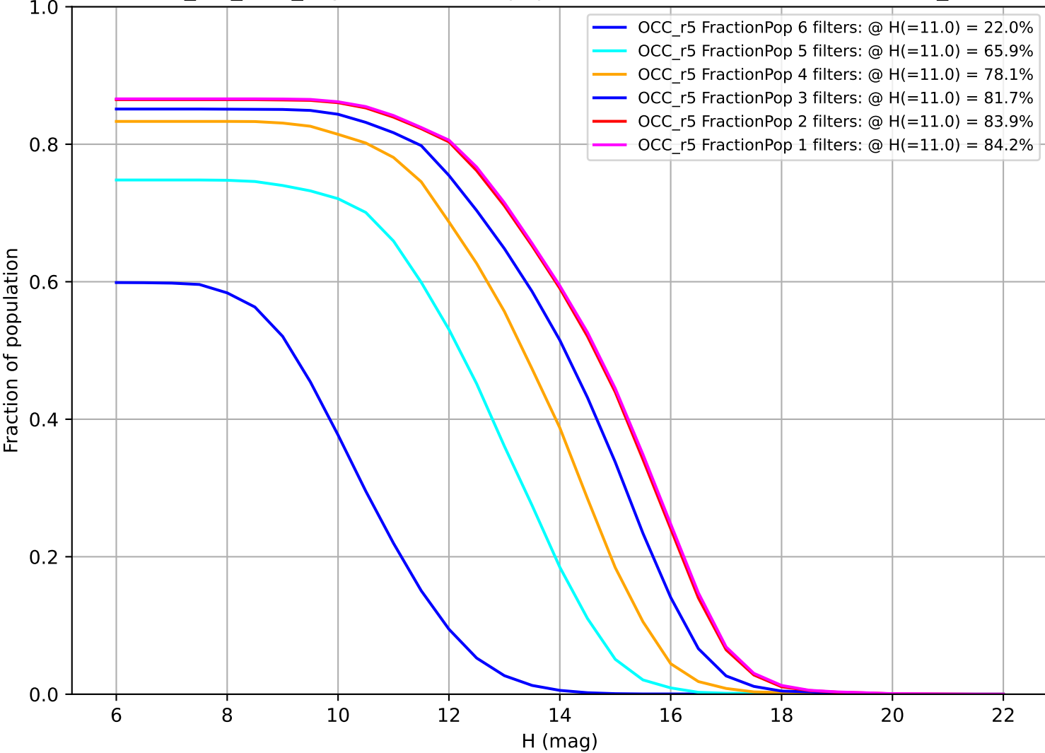
ddf_roll_v3.5_10yrs: Fraction of population with colors in X filters OCC_r5
