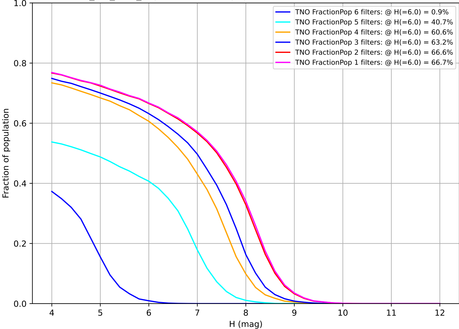
ddf_roll_v3.5_10yrs: Fraction of population with colors in X filters TNO
