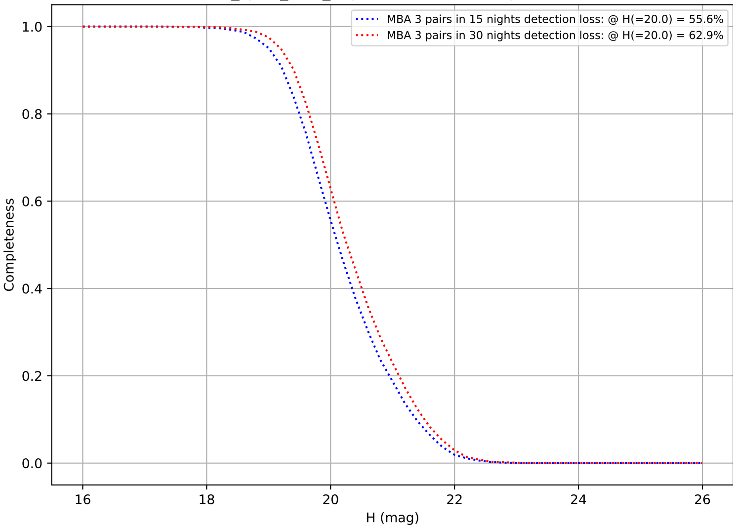
four_cycle_v3.5_10yrs: DifferentialCompleteness
